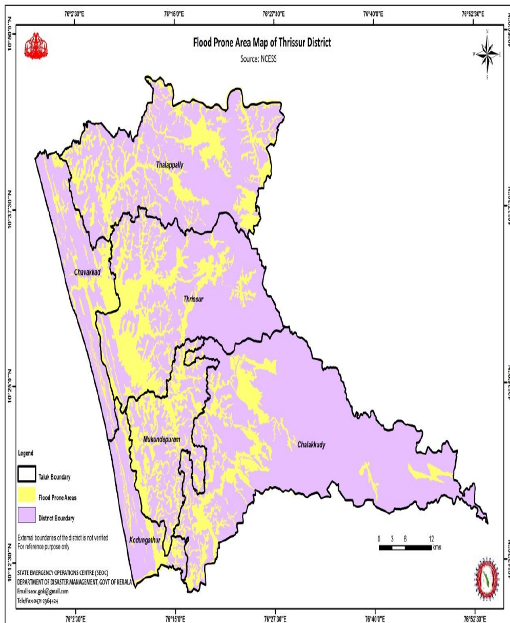
FIGURE 10: FLOOD PRONE AREA MAP OF THRISSUR DISTRICT (ANNEXURE 26)
