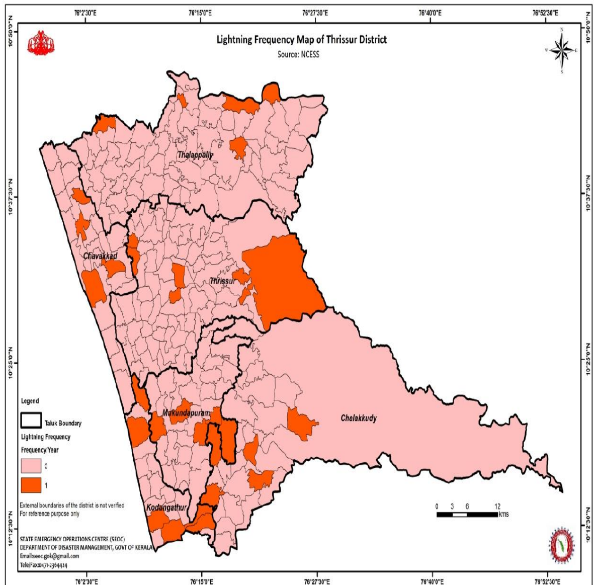
FIGURE 13: LIGHTNING FREQUENCY MAP OF THRISSUR DISTRICT (ANNEXURE 27)
