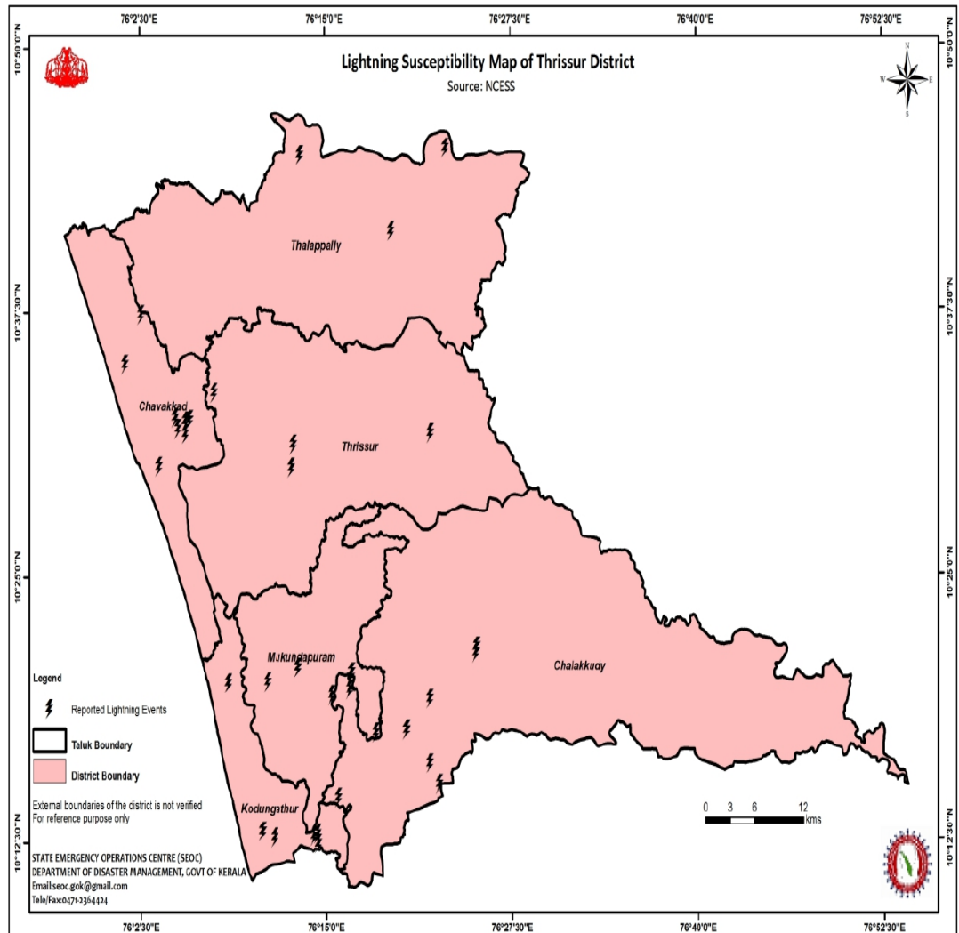
FIGURE 14: LIGHTNING SUSCEPTIBILITY MAP OF THRISSUR DISTRICT (ANNEXURE 28)
