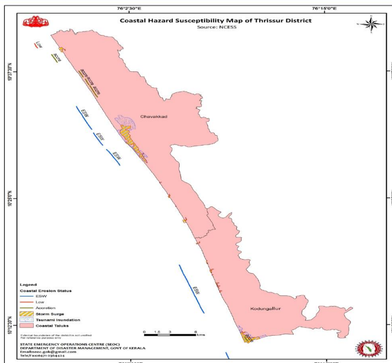
FIGURE 16: COASTAL HAZARD SUSCEPTIBILITY MAP OF THRISSUR DISTRICT
