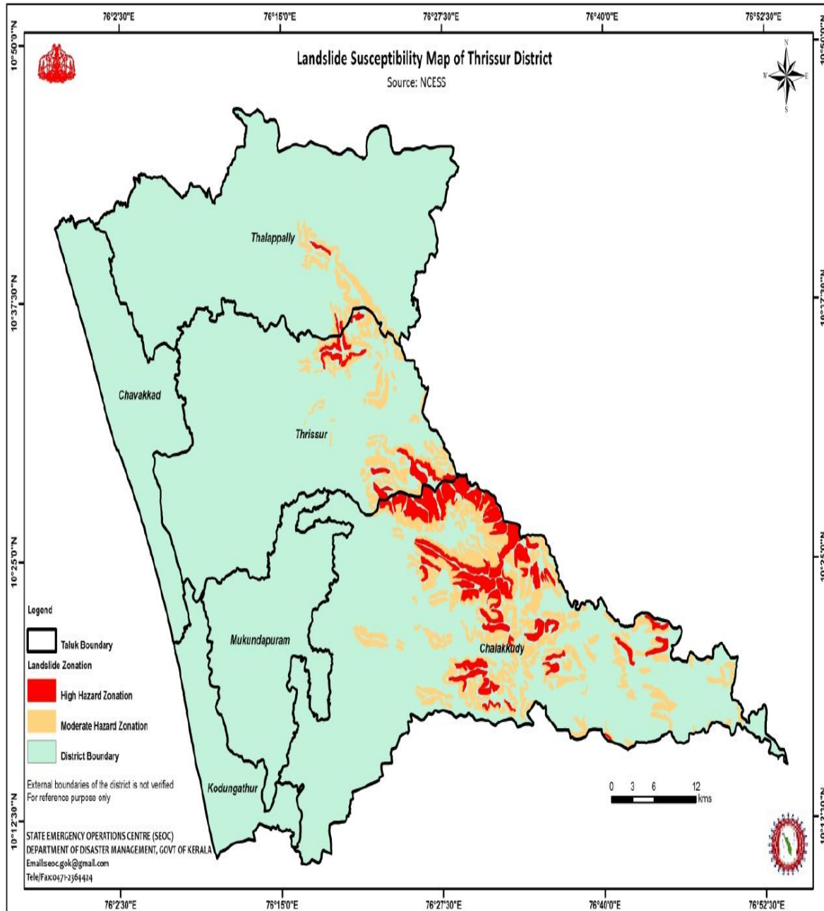
FIGURE 11: LANDSLIDE SUSCEPTIBILITY MAP OF THRISSUR DISTRICT (ANNEXURE 26)
