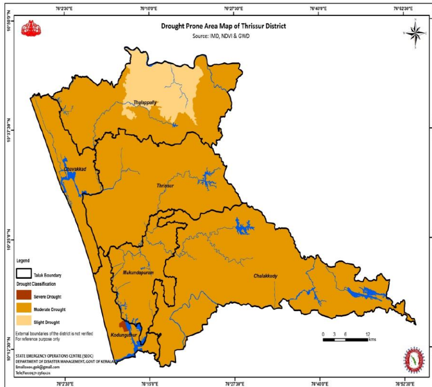
FIGURE 15: DROUGHT PRONE AREA MAP OF THRISSUR DISTRICT (ANNEXURE 29)
