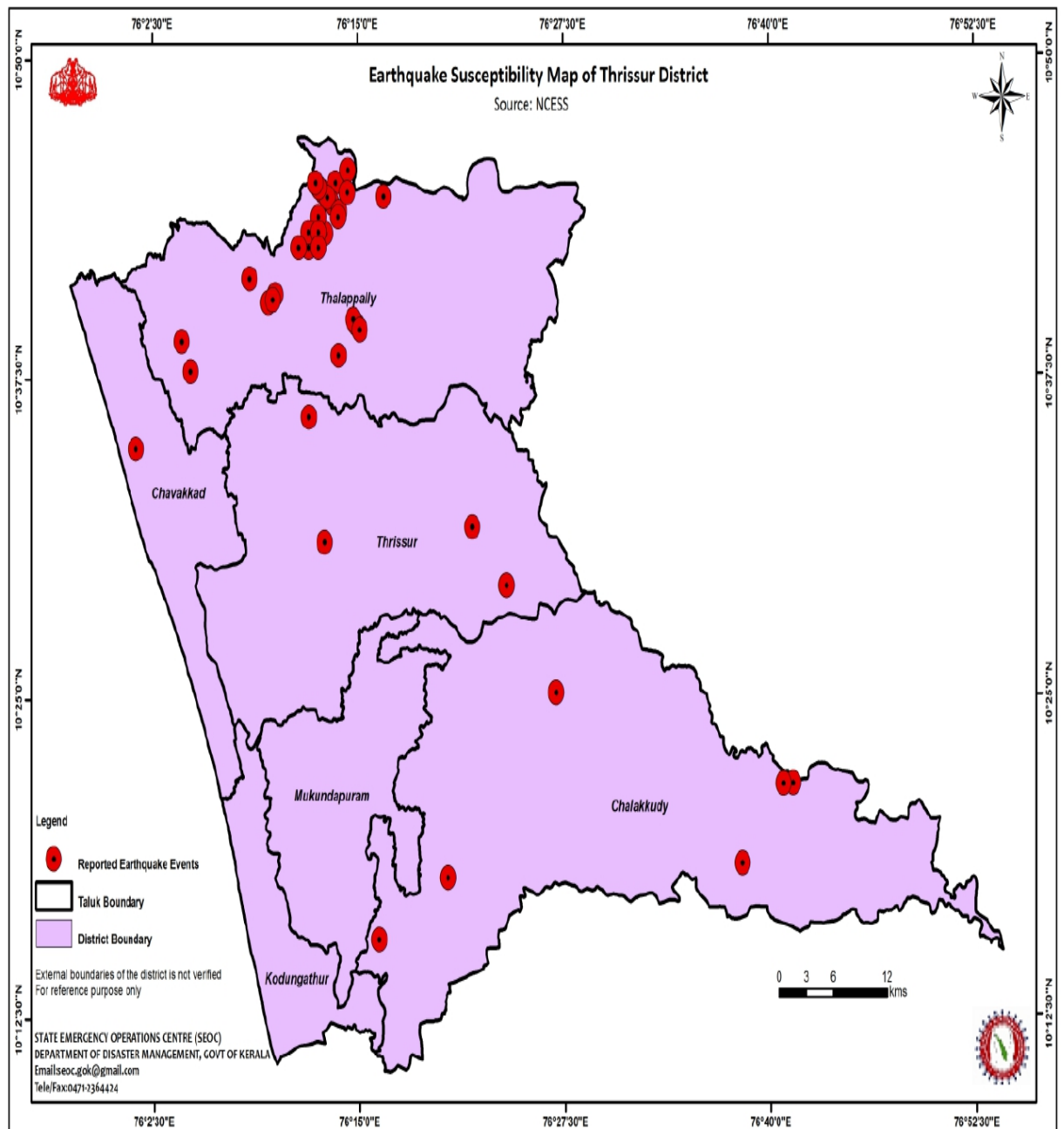
FIGURE 12: EARTHQUAKE SUSCEPTIBILITY MAP OF THRISSUR DISTRICT
